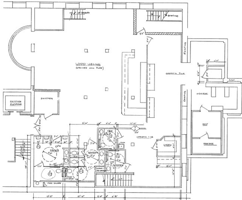
Lower Level
